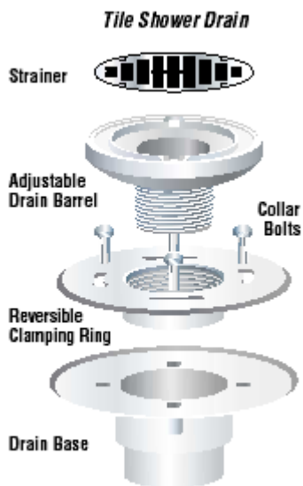
Three-Piece Drain
