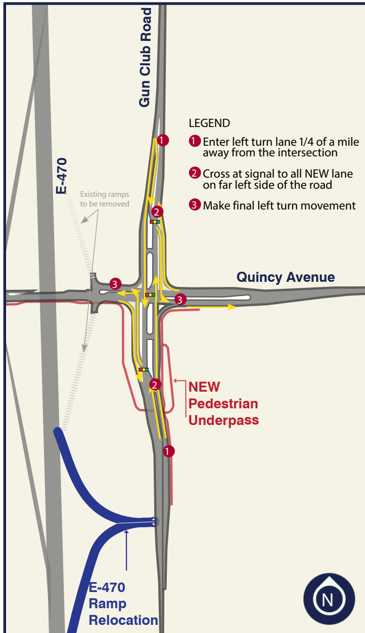
New PCFI Intersection Configuration
